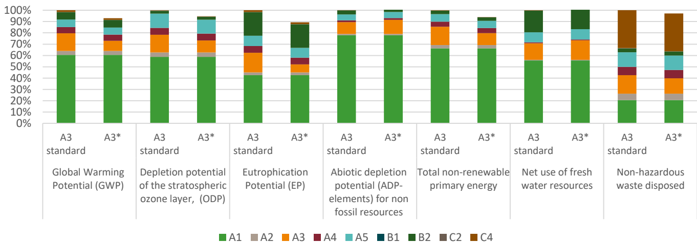
Figure 4: Graph depicting selection of impact indicator results calculated according to EN 15804
